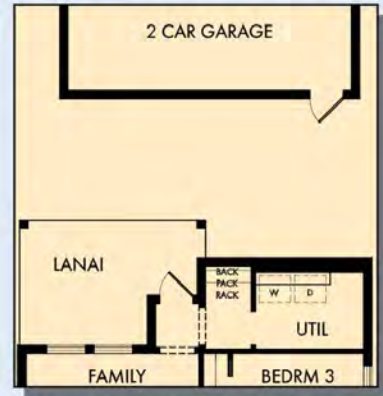
FIRST FLOOR WITH OPTIONAL DETACHED 2 CAR GARAGE
