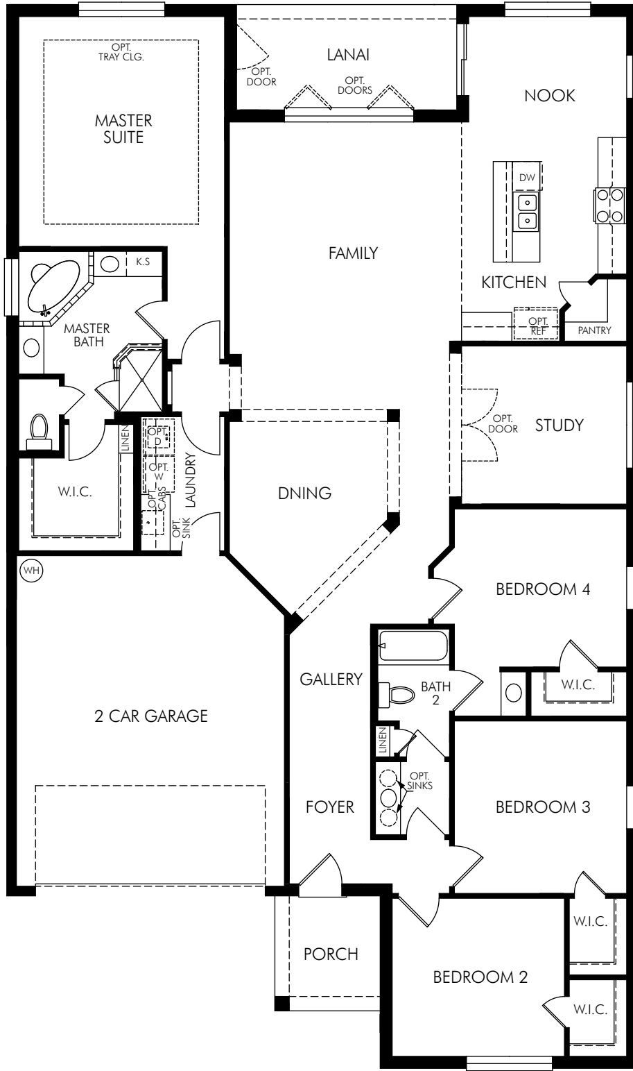
FLOOR PLAN
